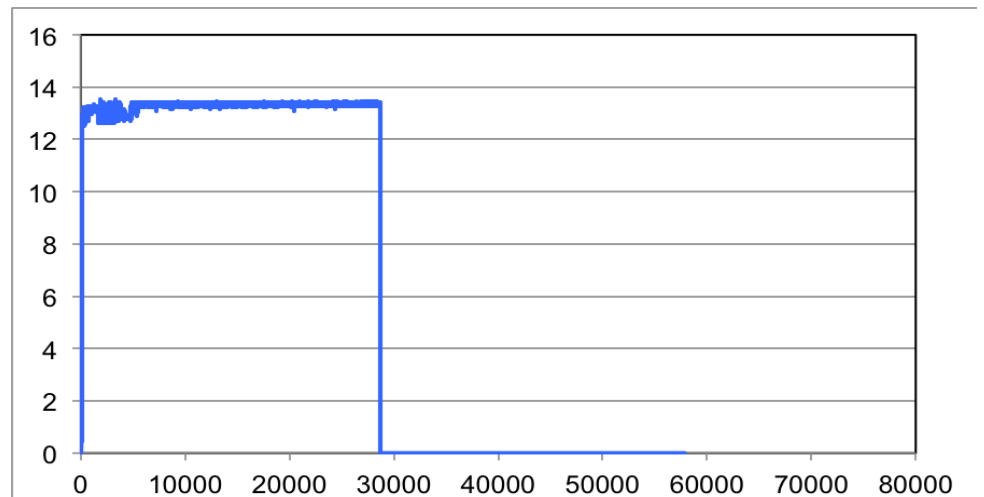
Charging curve for Leaf showing current fluctuation at beginning of charging cycle 1_0128 (July 12, 2013)
